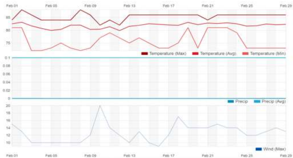
Figure 5 Monthly temperature, precipitation and wind in February 2020.
