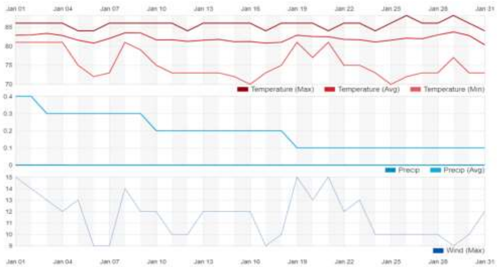
Figure 4 Monthly temperature, precipitation and wind in January 2020.
